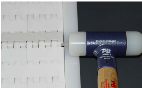
Hammer in the rod head
