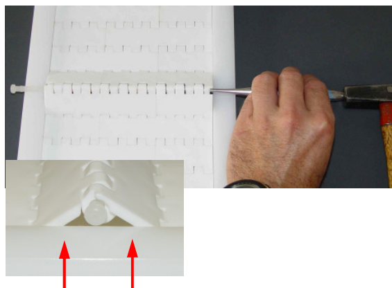
Leverage rod head out
